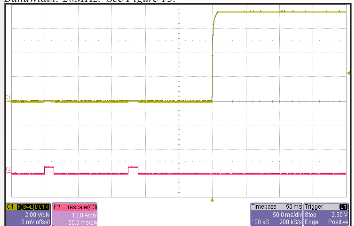
Figure 16: Rise of output voltage after the removal of a short circuit across the output terminals. Ch 1: V_{out} (2V/div). F 2: I_{out} (10A/div).
