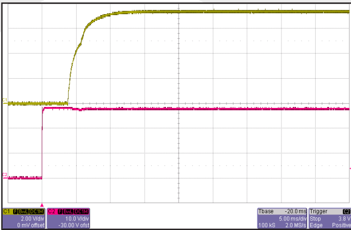
Figure 9: Turn-on transient at full resistive load and zero output capacitance initiated by Vin. ENA1 previously high. Ch 1: Vout (2V/div). Ch 2: Vin (10V/div).
