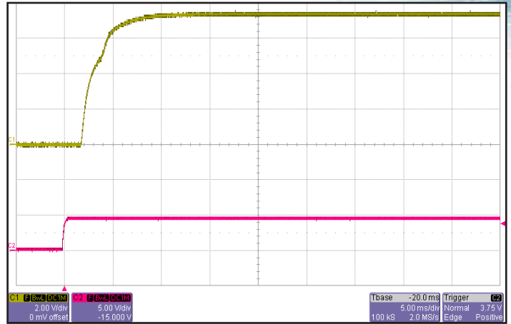
Figure 8: Turn-on transient at full resistive load and 400uF output capacitance initiated by ENA1. Input voltage pre-applied. Ch 1: Vout (2V/div). Ch 2: ENA1 (5V/div).
