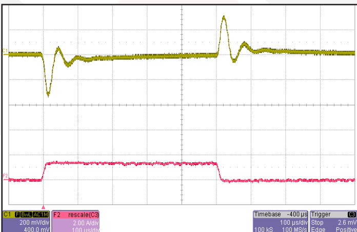
Figure 11: Output voltage response to step-change in load current 0%-50%-0% of Iout (max). Load cap: 1uF ceramic cap and 10uF, 100mΩ ESR tantalum cap. Ch 1: Vout (200mV/div). Ch 2: Iout (2A/div).
