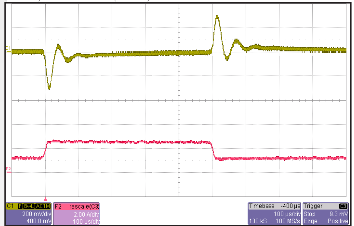
Figure 10: Output voltage response to step-change in load current 50%-100%-50% of Iout (max). Load cap: 1uF ceramic cap and 10uF, 100mΩ ESR tantalum cap. Ch 1: Vout (200mV/div). Ch 2: Iout (2A/div).
